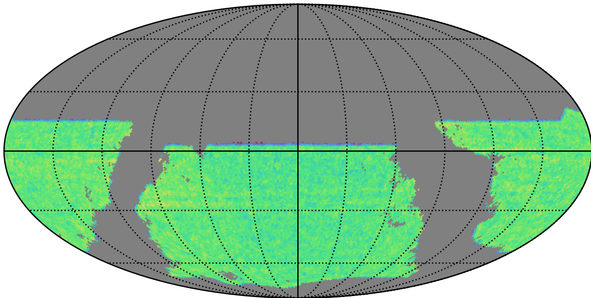
octo_v3.4_10yrs gri band non-DD: WeakLensingNvisits
