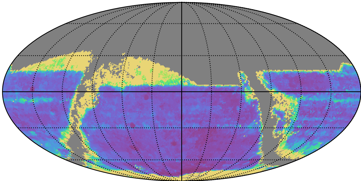
octo_v3.4_10yrs : TDC_accuracy
