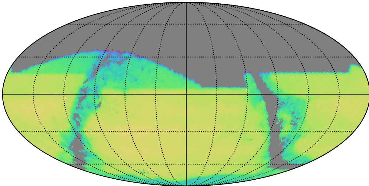
octo_v3.4_10yrs z band and non-DD: QSONumberCountsMetric
