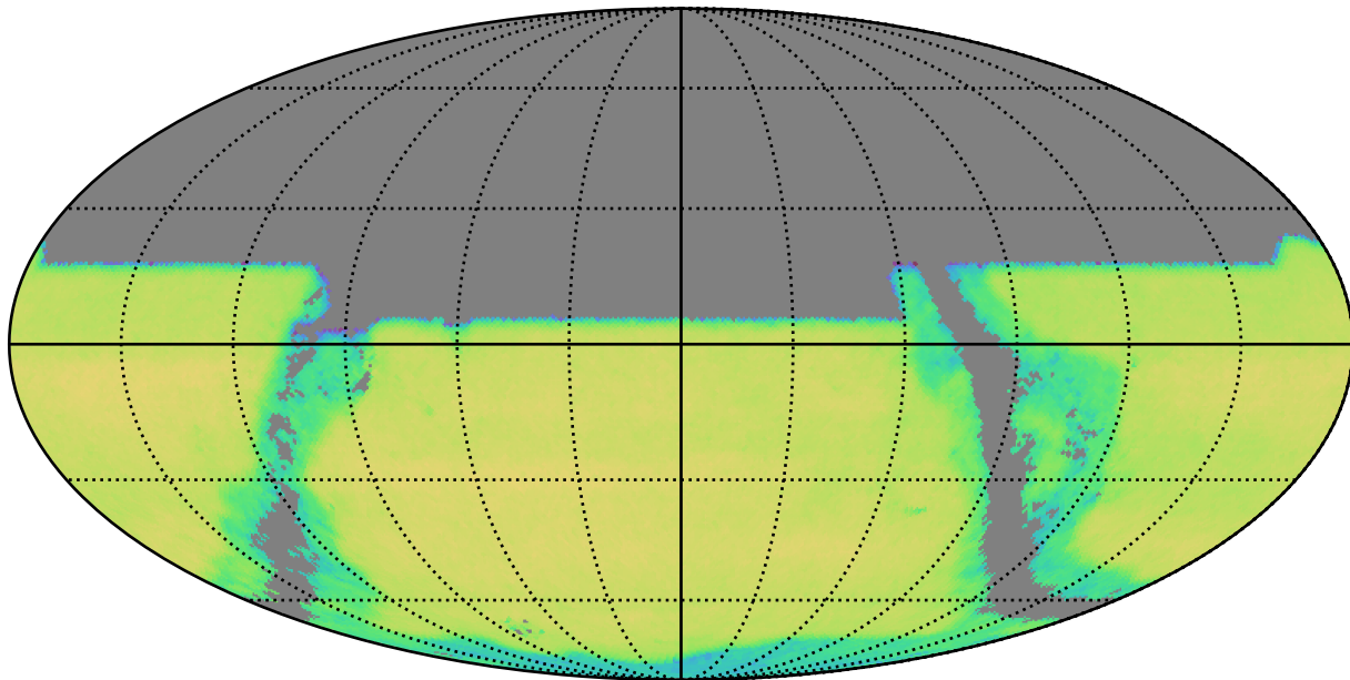
octo_v3.4_10yrs y band and non-DD: QSONumberCountsMetric
