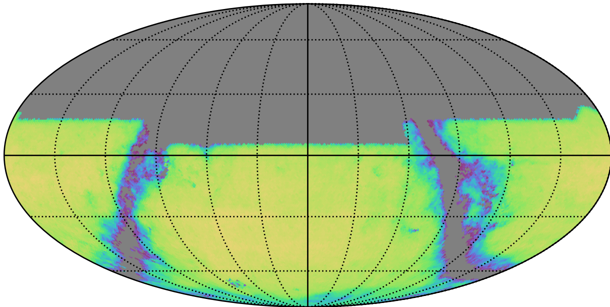
octo_v3.4_10yrs u band and non-DD: QSONumberCountsMetric
