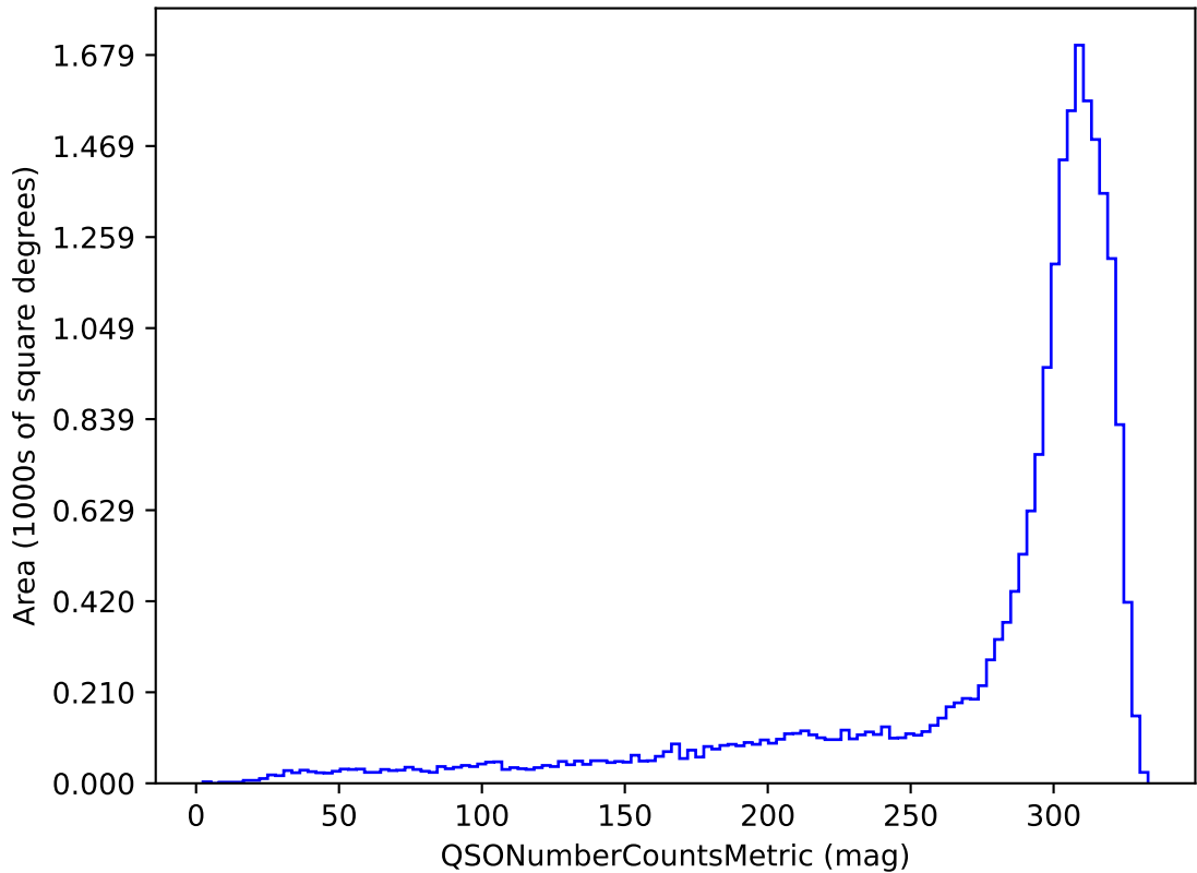
octo_v3.4_10yrs u band and non-DD: QSONumberCountsMetric
