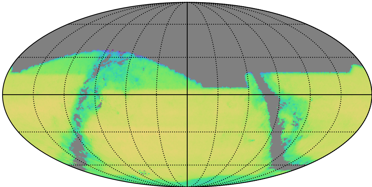
octo_v3.4_10yrs i band and non-DD: QSONumberCountsMetric
