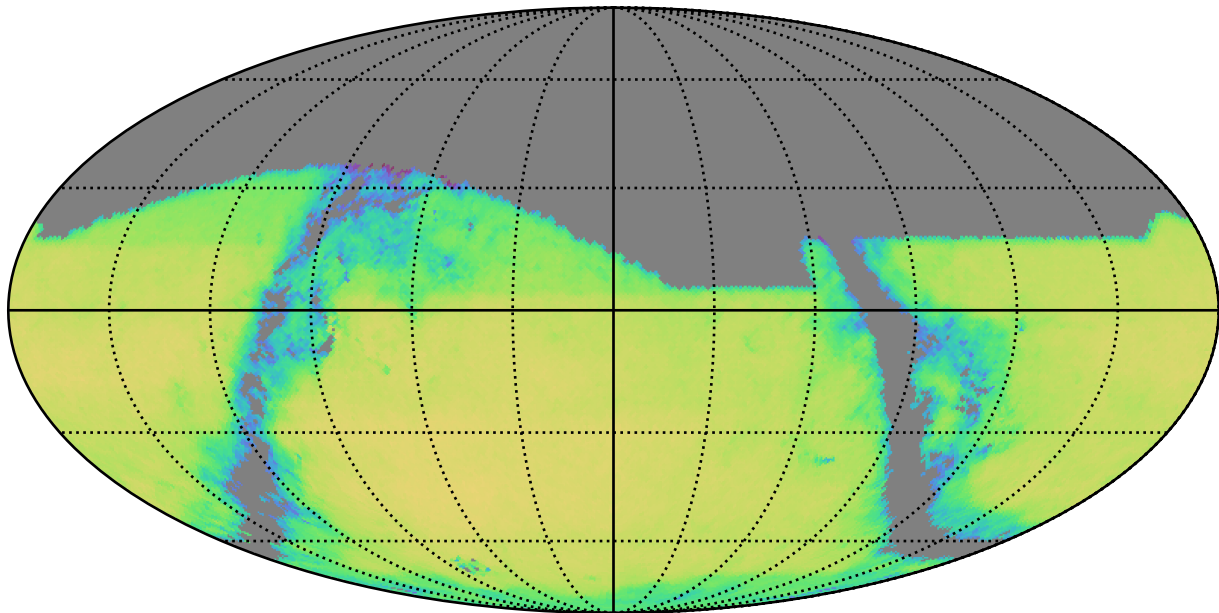
octo_v3.4_10yrs g band and non-DD: QSONumberCountsMetric
