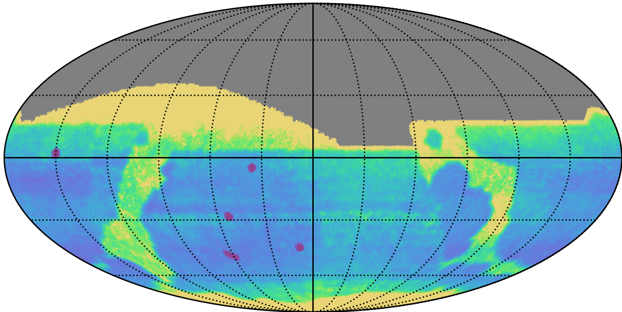
octo_v3.4_10yrs : Proper Motion Uncert @ 24.0
