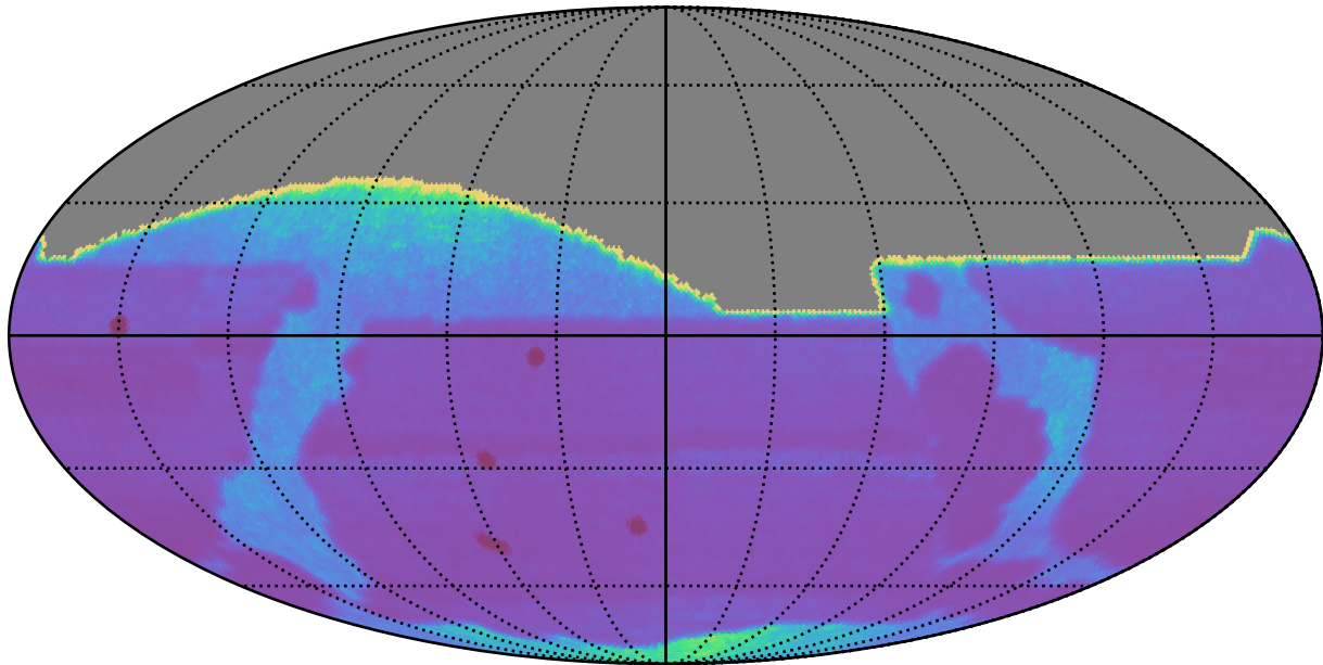
octo_v3.4_10yrs : Proper Motion Uncert @ 20.5
