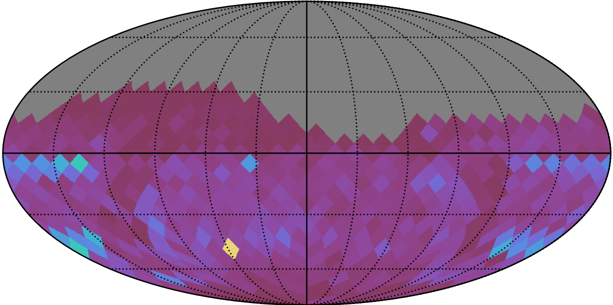
octo_v3.4_10yrs dm 21 interval 30 R Rc Year 1-2: PeriodicStarModulationMetric
