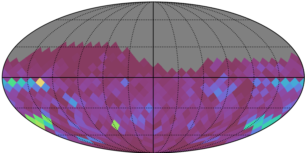
octo_v3.4_10yrs dm 21 interval 15 RRC Year 1-2: PeriodicStarModulationMetric
