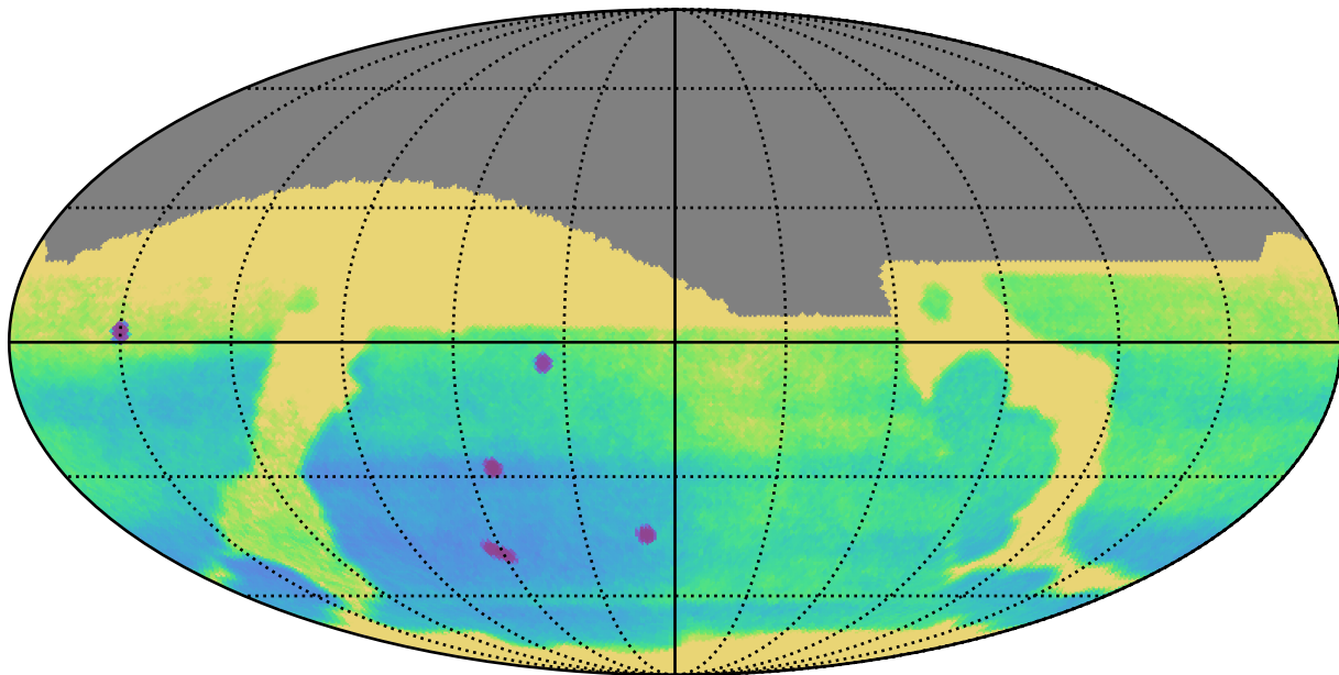
octo_v3.4_10yrs : Parallax Uncert @ 24.0
