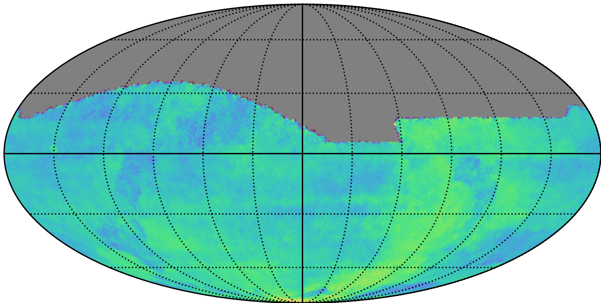
octo_v3.4_10yrs : Parallax Coverage @ 24.0
