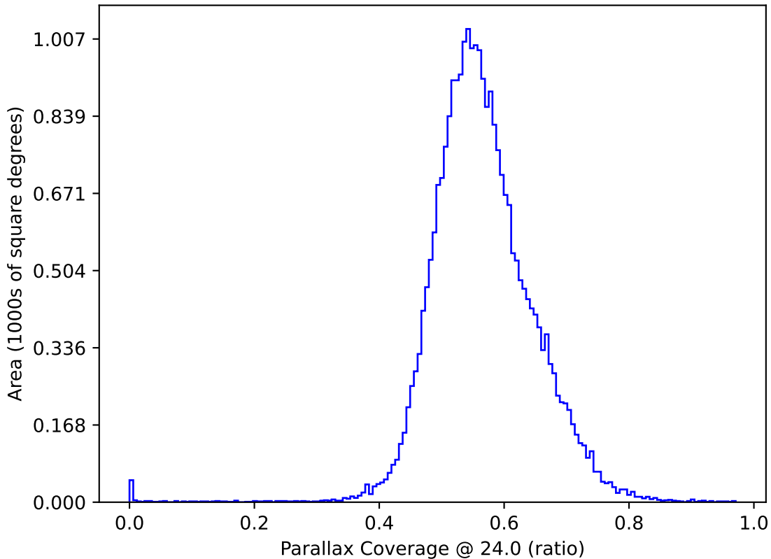
octo_v3.4_10yrs : Parallax Coverage @ 24.0
