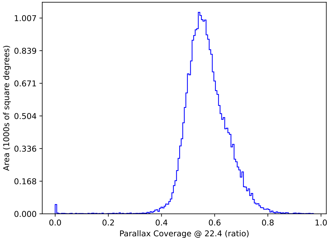
octo_v3.4_10yrs : Parallax Coverage @ 22.4
