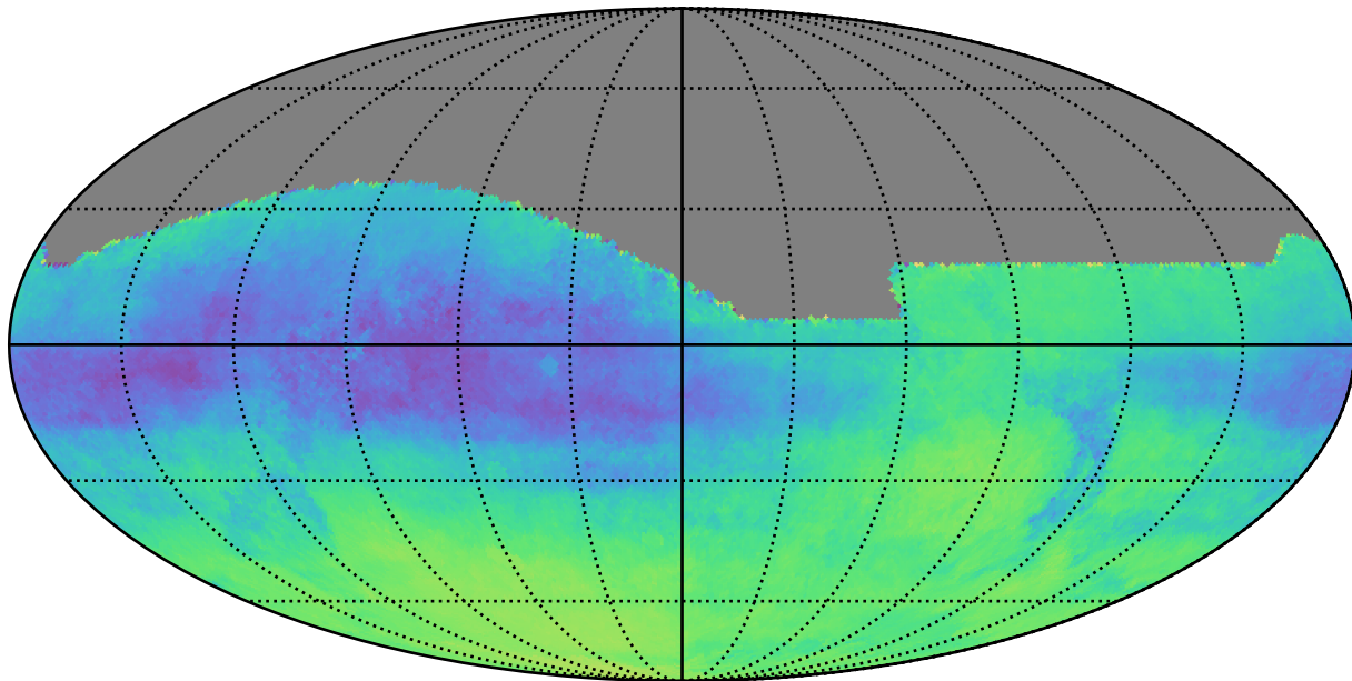
octo_v3.4_10yrs : Parallax-DCR degeneracy @ 24.0
