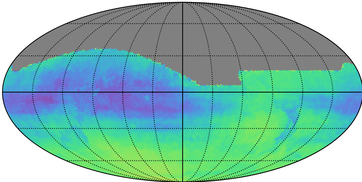
octo_v3.4_10yrs : Parallax-DCR degeneracy @ 22.4
