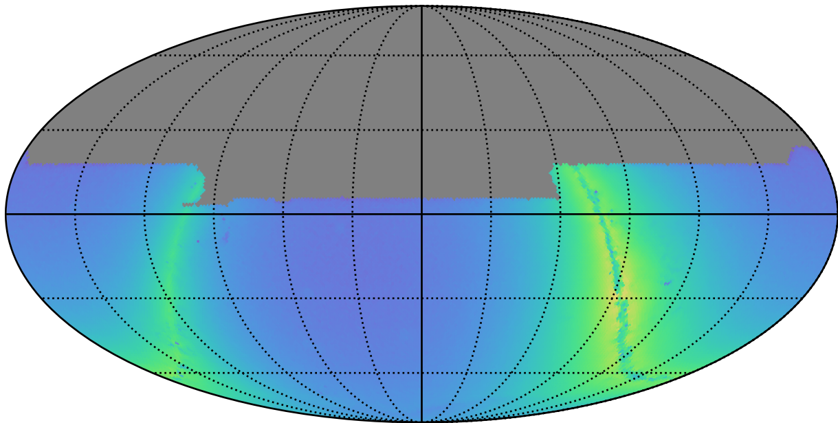
octo_v3.4_10yrs y: Nstars_no_crowding
