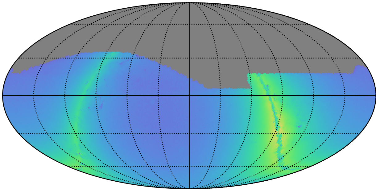
octo_v3.4_10yrs r: Nstars_no_crowding
