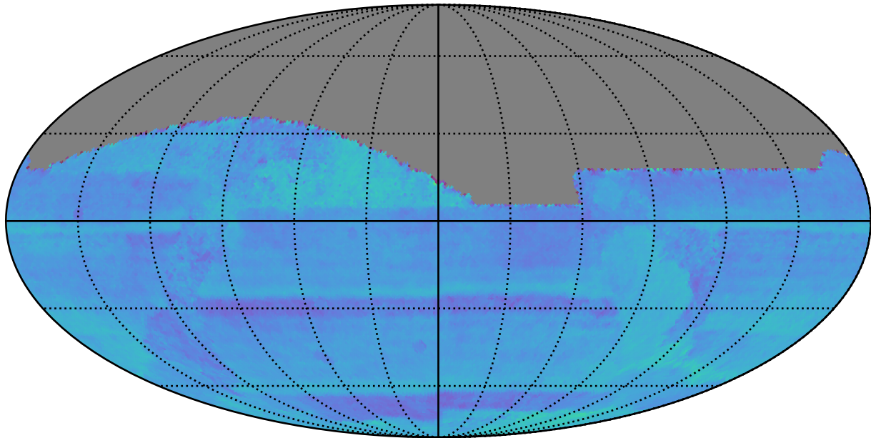
octo_v3.4_10yrs : Normalized Proper Motion Uncert @ 24.0
