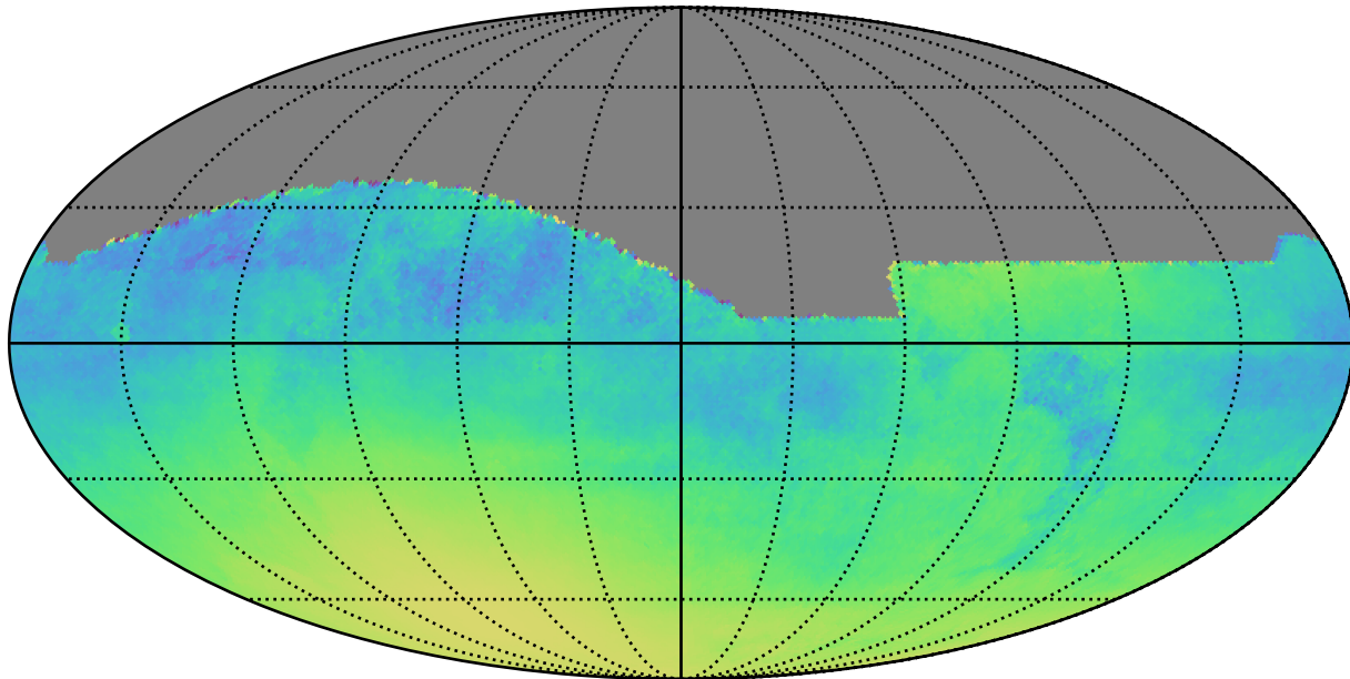
octo_v3.4_10yrs : Normalized Parallax Uncert @ 24.0
