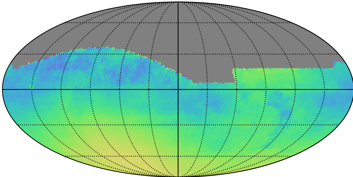
octo_v3.4_10yrs : Normalized Parallax Uncert @ 22.4
