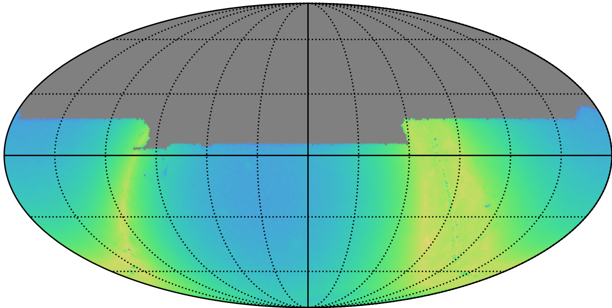
octo_v3.4_10yrs y: N stars to Precision 0.20
