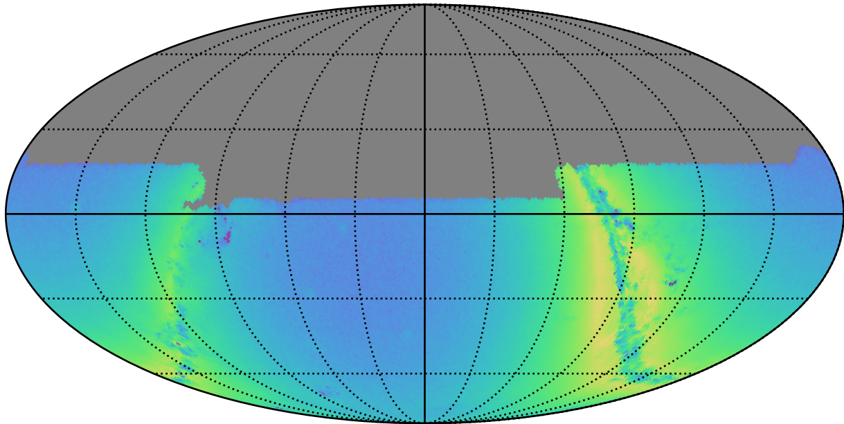
octo_v3.4_10yrs u: N stars to Precision 0.20
