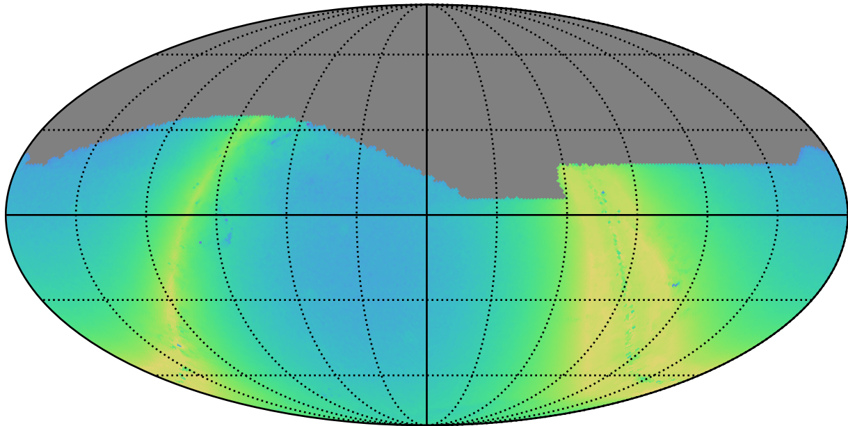
octo_v3.4_10yrs r: N stars to Precision 0.20
