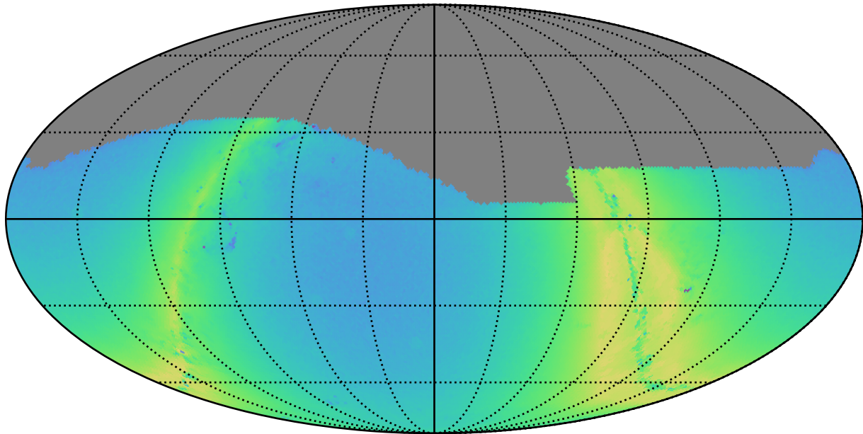
octo_v3.4_10yrs g: N stars to Precision 0.20
