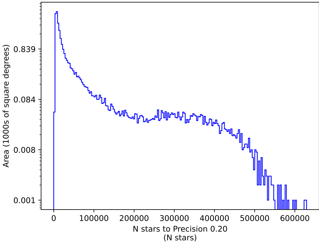
octo_v3.4_10yrs g: N stars to Precision 0.20
