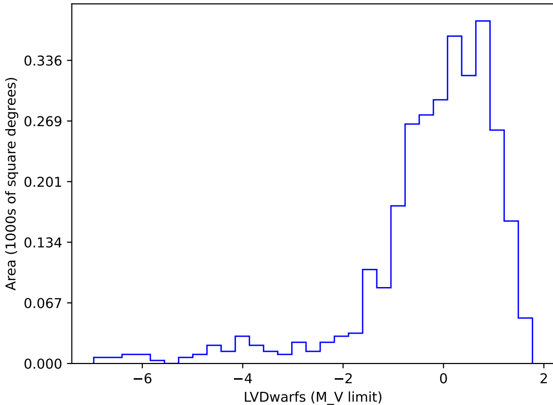
octo_v3.4_10yrs gi SCP: LVDwarfs
