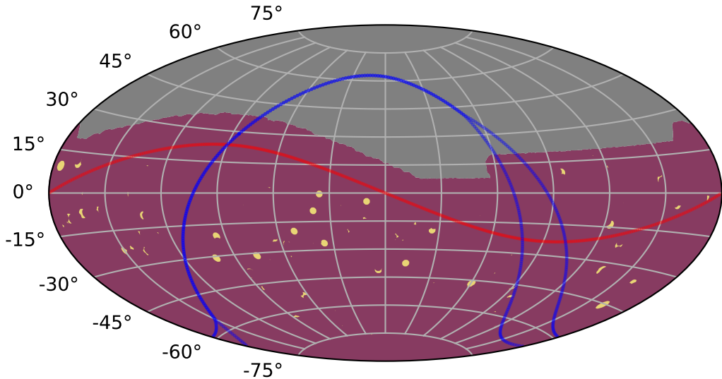
octo_v3.4_10yrs all models: KNePopMetric_all_ztfrest_simple_blue
