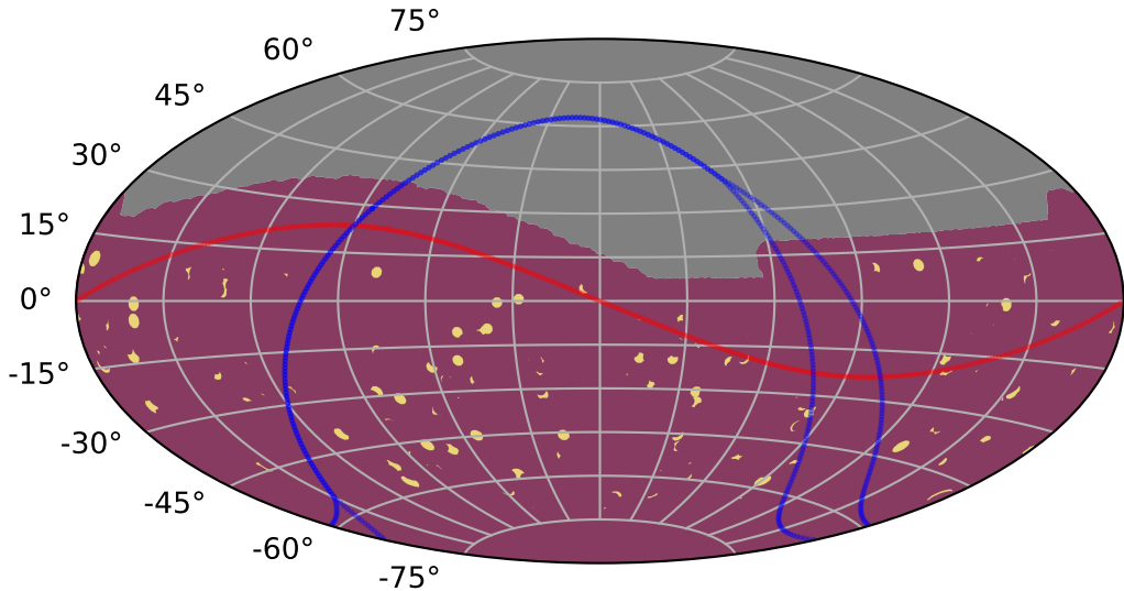
octo_v3.4_10yrs all models: KNePopMetric_all_red_color_detect
