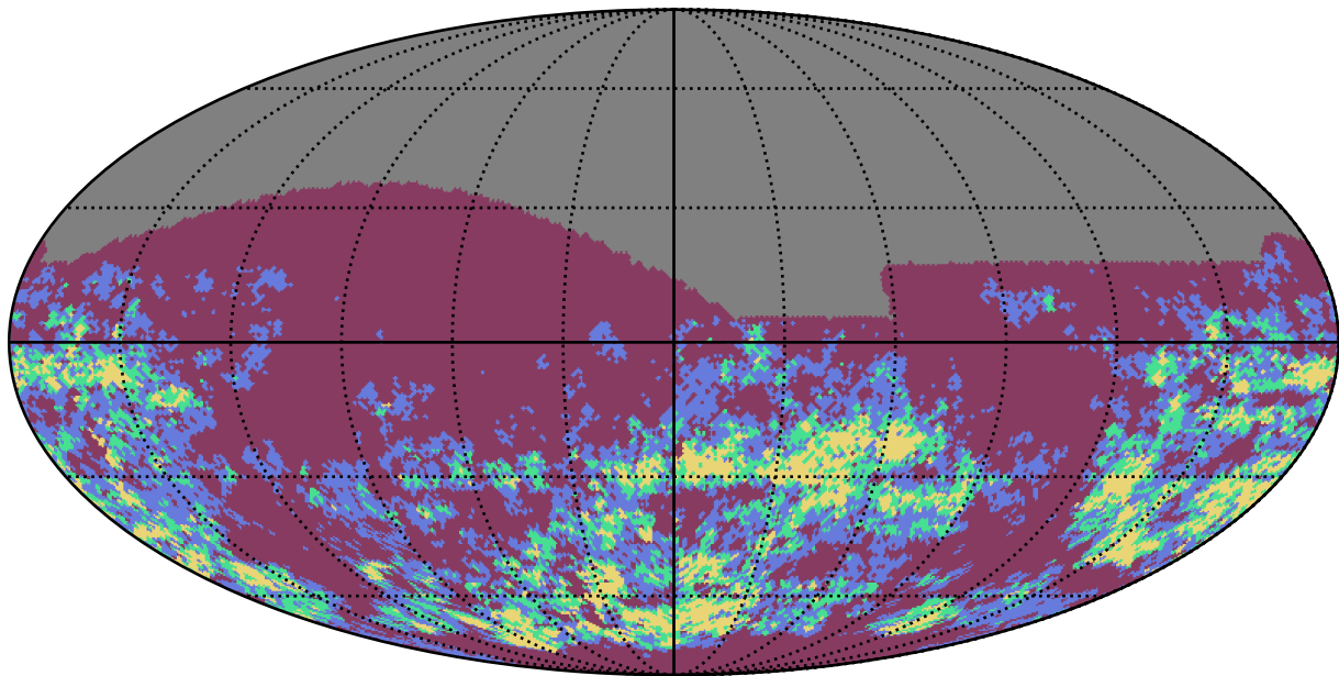
octo_v3.4_10yrs z band: Gaps_7hr
