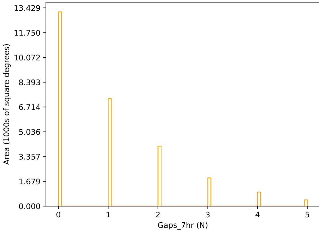
octo_v3.4_10yrs r band: Gaps_7hr
