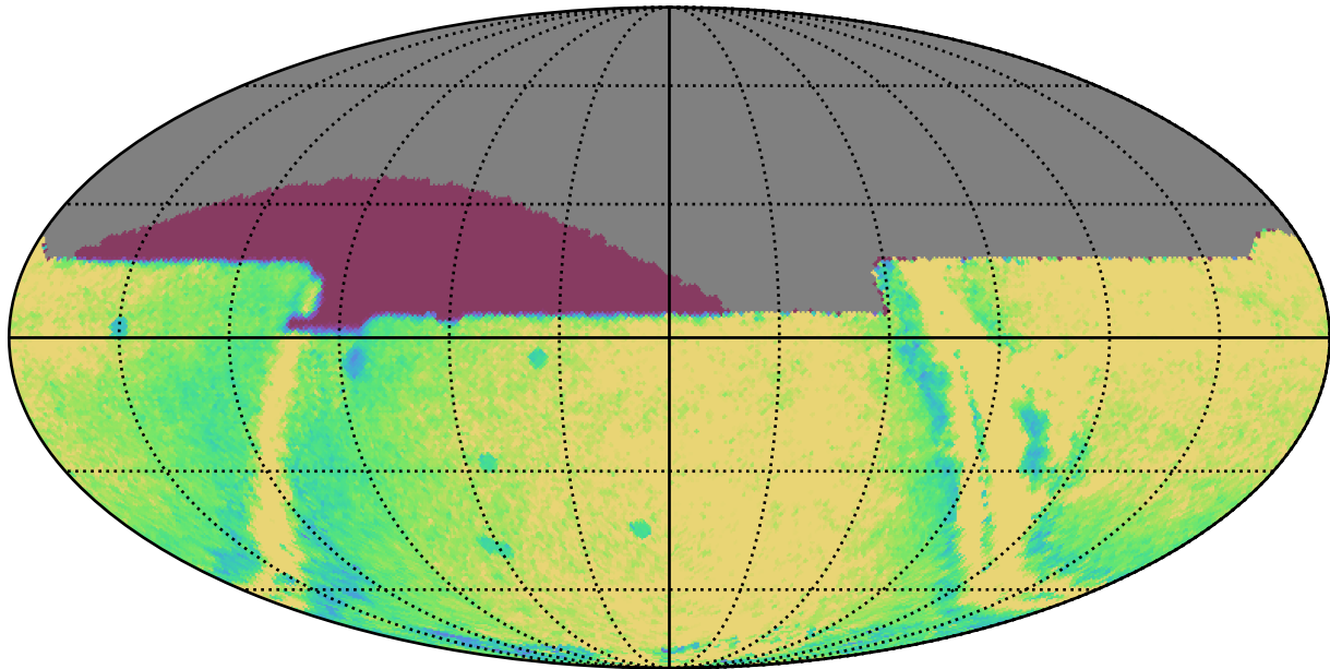
octo_v3.4_10yrs : GalplaneTimePerFilter_xray_binaries_map_y
