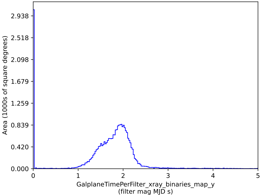
octo_v3.4_10yrs : GalplaneTimePerFilter_xray_binaries_map_y
