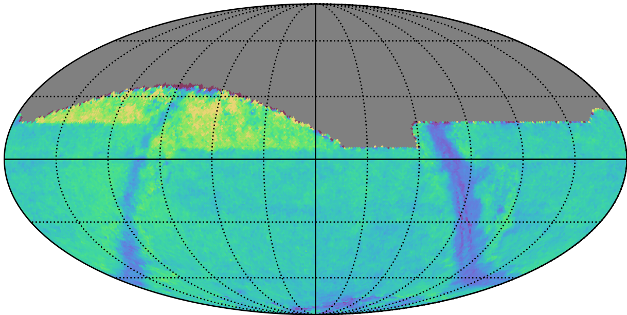
octo_v3.4_10yrs : GalplaneTimePerFilter_xray_binaries_map_i
