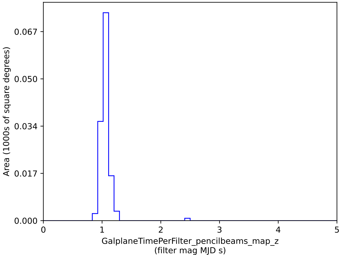
octo_v3.4_10yrs : GalplaneTimePerFilter_pencilbeams_map_z
