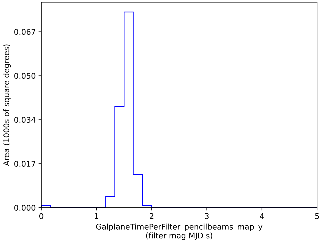
octo_v3.4_10yrs : GalplaneTimePerFilter_pencilbeams_map_y
