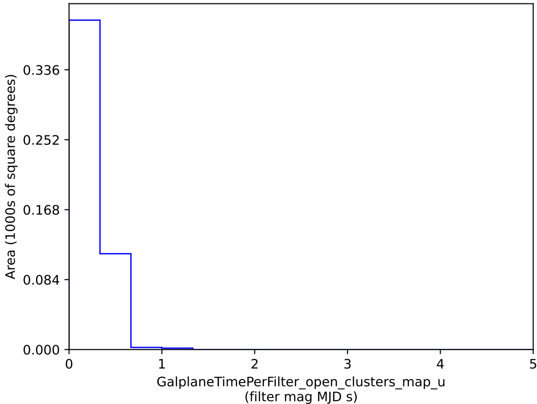
octo_v3.4_10yrs : GalplaneTimePerFilter_open_clusters_map_u
