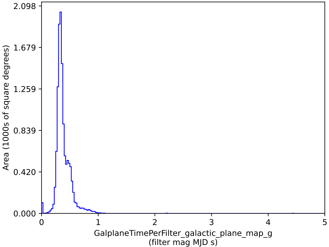
octo_v3.4_10yrs : GalplaneTimePerFilter_galactic_plane_map_g
