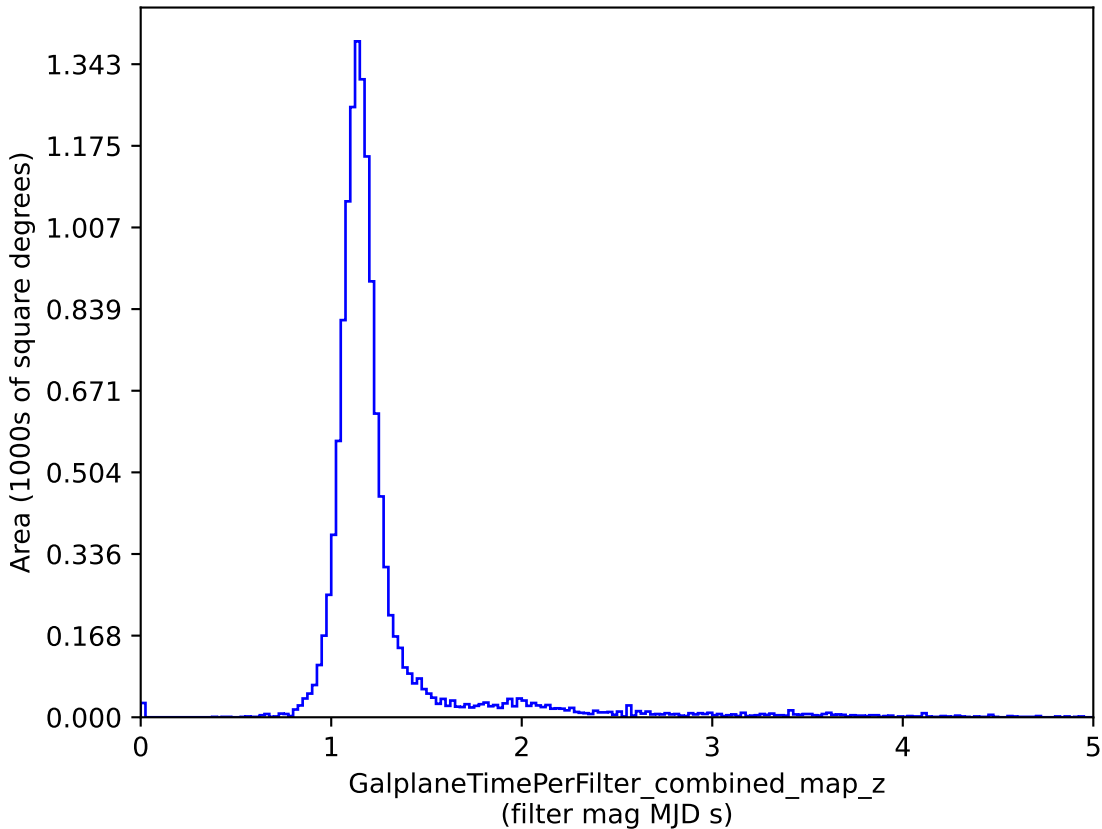
octo_v3.4_10yrs : GalplaneTimePerFilter_combined_map_z
