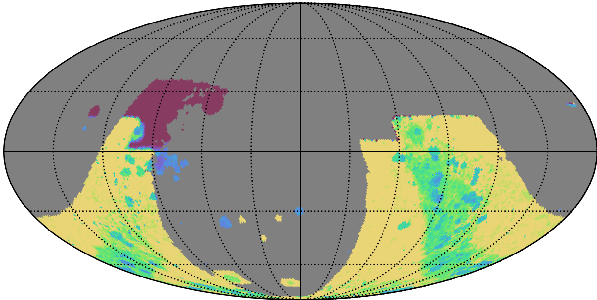
octo_v3.4_10yrs : GalplaneTimePerFilter_combined_map_y
