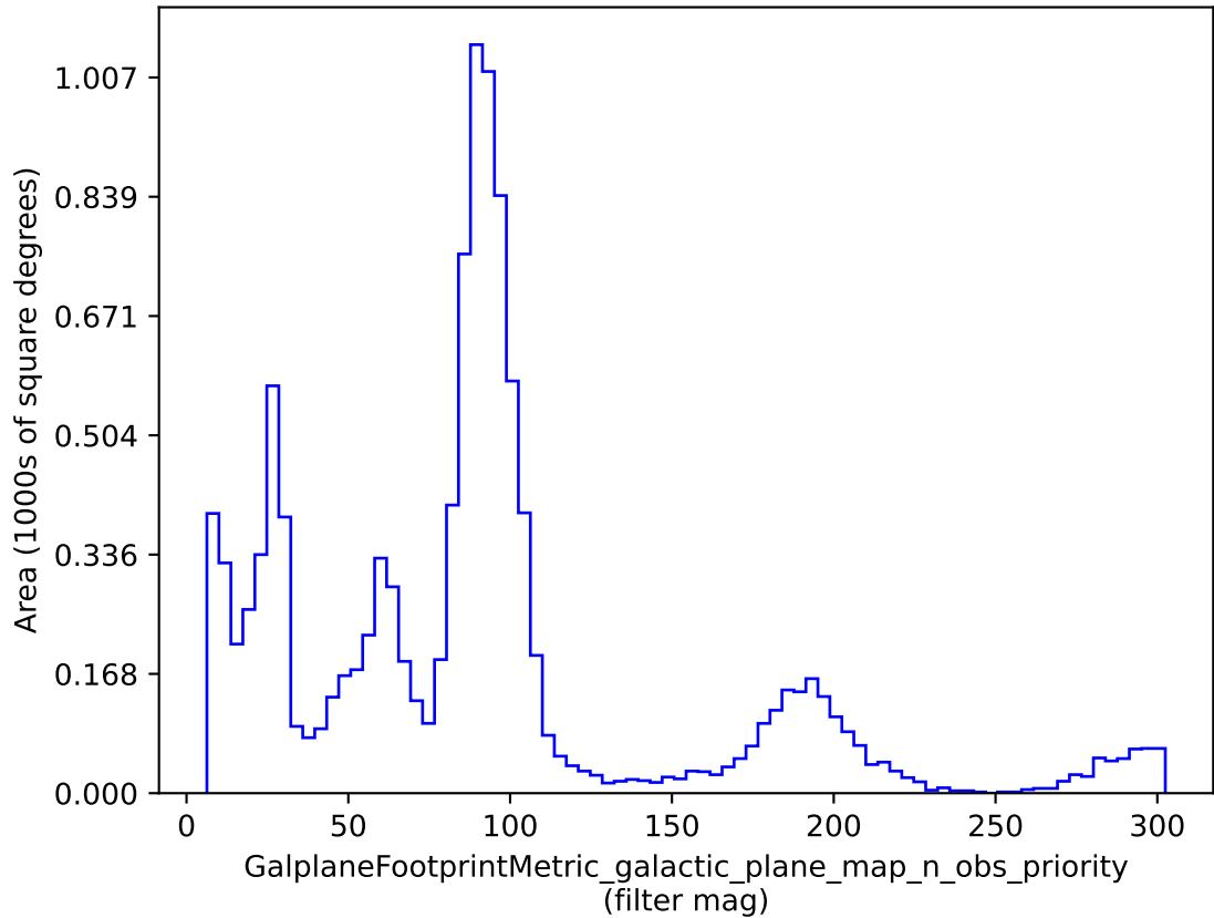
octo_v3.4_10yrs : GalplaneFootprintMetric_galactic_plane_map_n_obs_priority
