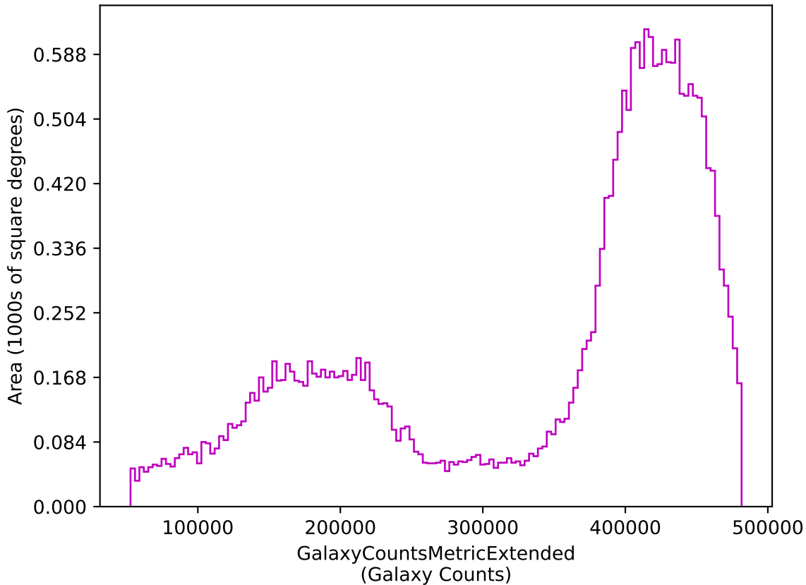
octo_v3.4_10yrs z: GalaxyCountsMetricExtended
