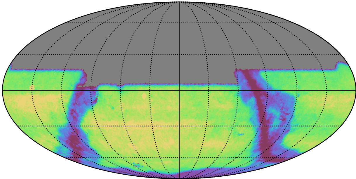
octo_v3.4_10yrs y: GalaxyCountsMetricExtended
