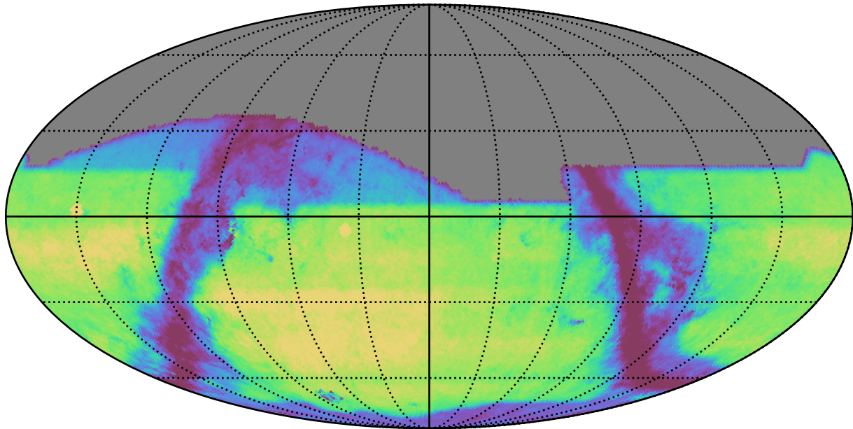
octo_v3.4_10yrs r: GalaxyCountsMetricExtended
