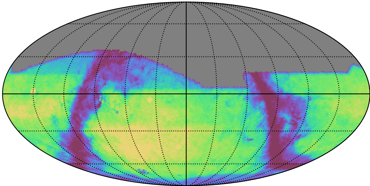
octo_v3.4_10yrs g: GalaxyCountsMetricExtended
