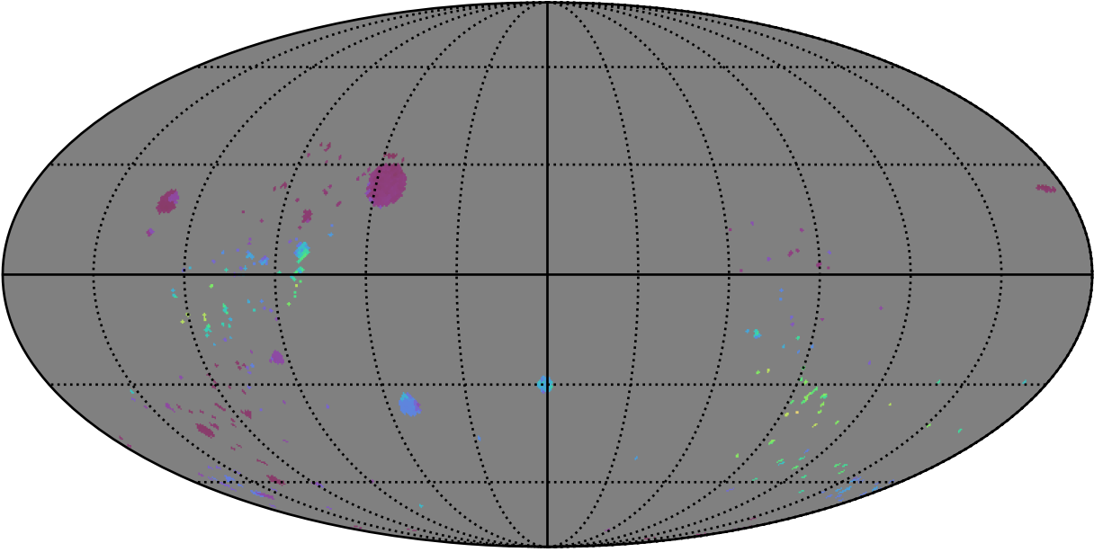
octo_v3.4_10yrs : GalPlaneSeasonGapsTimescales_open_clusters_map_Tau_55_0
