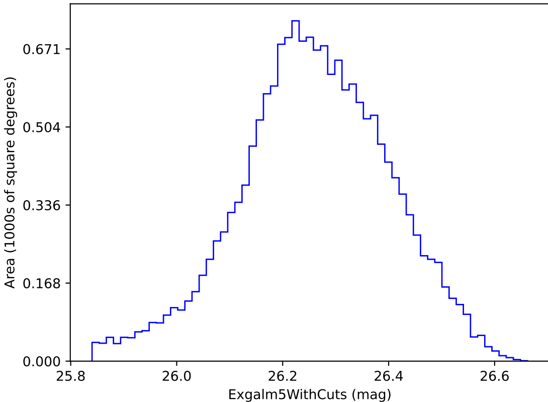
octo_v3.4_10yrs i band non-DD year 9: ExgalM5WithCuts
