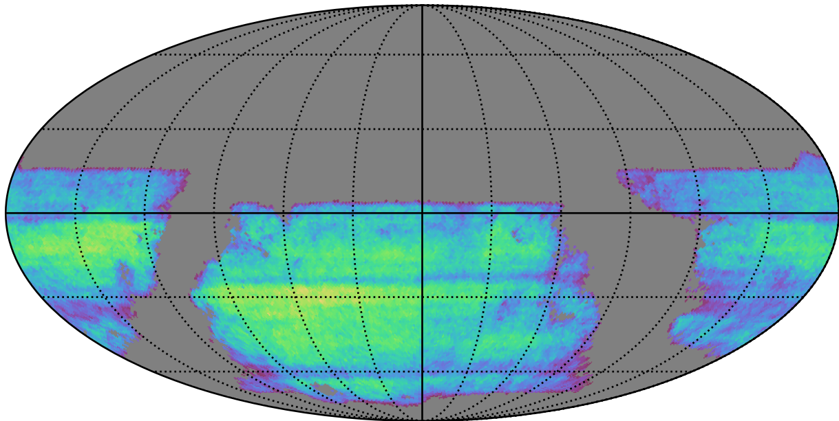
octo_v3.4_10yrs i band non-DD year 8: ExgalM5WithCuts
